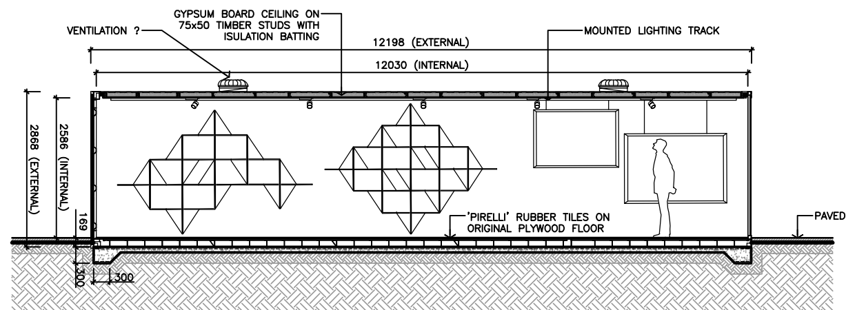
05 DT0040 SECTION 1:50
